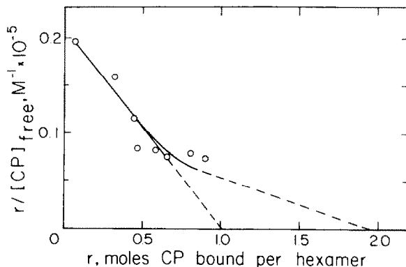
Fig. 3. Scatchard plot for the binding of chlorpromazine to GDH in the presence of 100 mM KCl, 2 mM \alpha KG and 0.1 M NADH. Conditions as described in Fig. 2.
